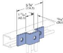
"U" Shape Bracket
