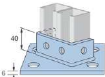
4 Hole Post Base
