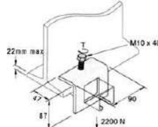
"Z" Shape Bracket
