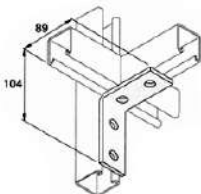
2 Hole Braced 90 Degree Angle
