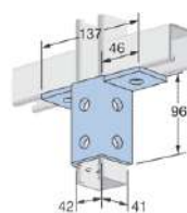
Electrical Hanger Fitting
