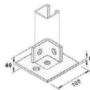
Square Saddle
