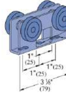
Trolley Assembly - 4 Wheel
