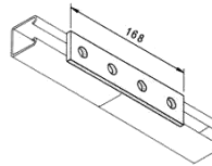
4 Hole Plate
