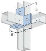
Angle Bracket (1359)
