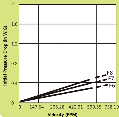
INITIAL RESTRICTION vs. FACE VELOCITY
